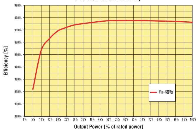
PVI-12.5-OUTD Efficiency
